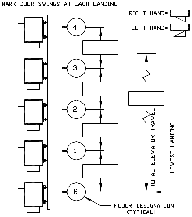
HOISTWAY ELEVATION VIEW
