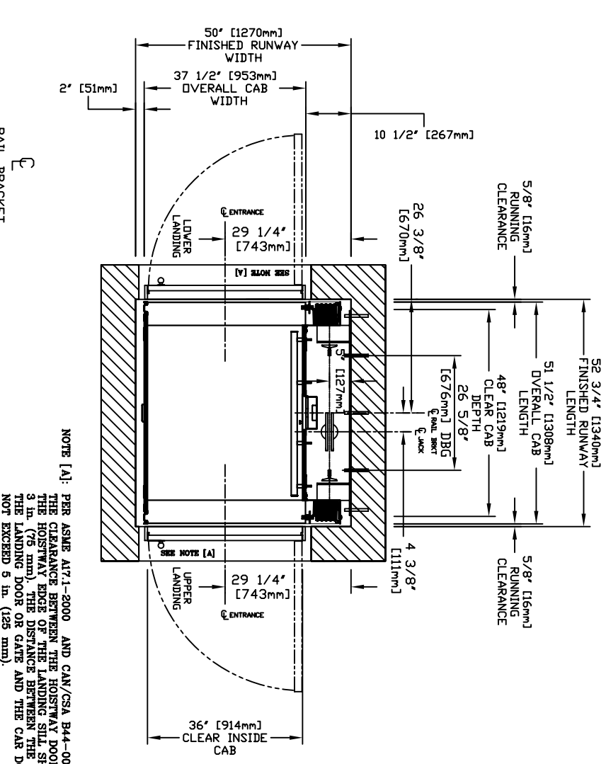
PLAN VIEW - INFINITY Model 3648 TYPE 2
